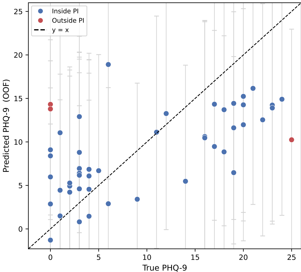
eGeMAPS + Whisper + Demo RMSE=6.81, R^2=0.343 (49/52 inside 95% PI)
