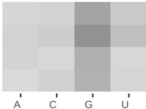
TadA- N
