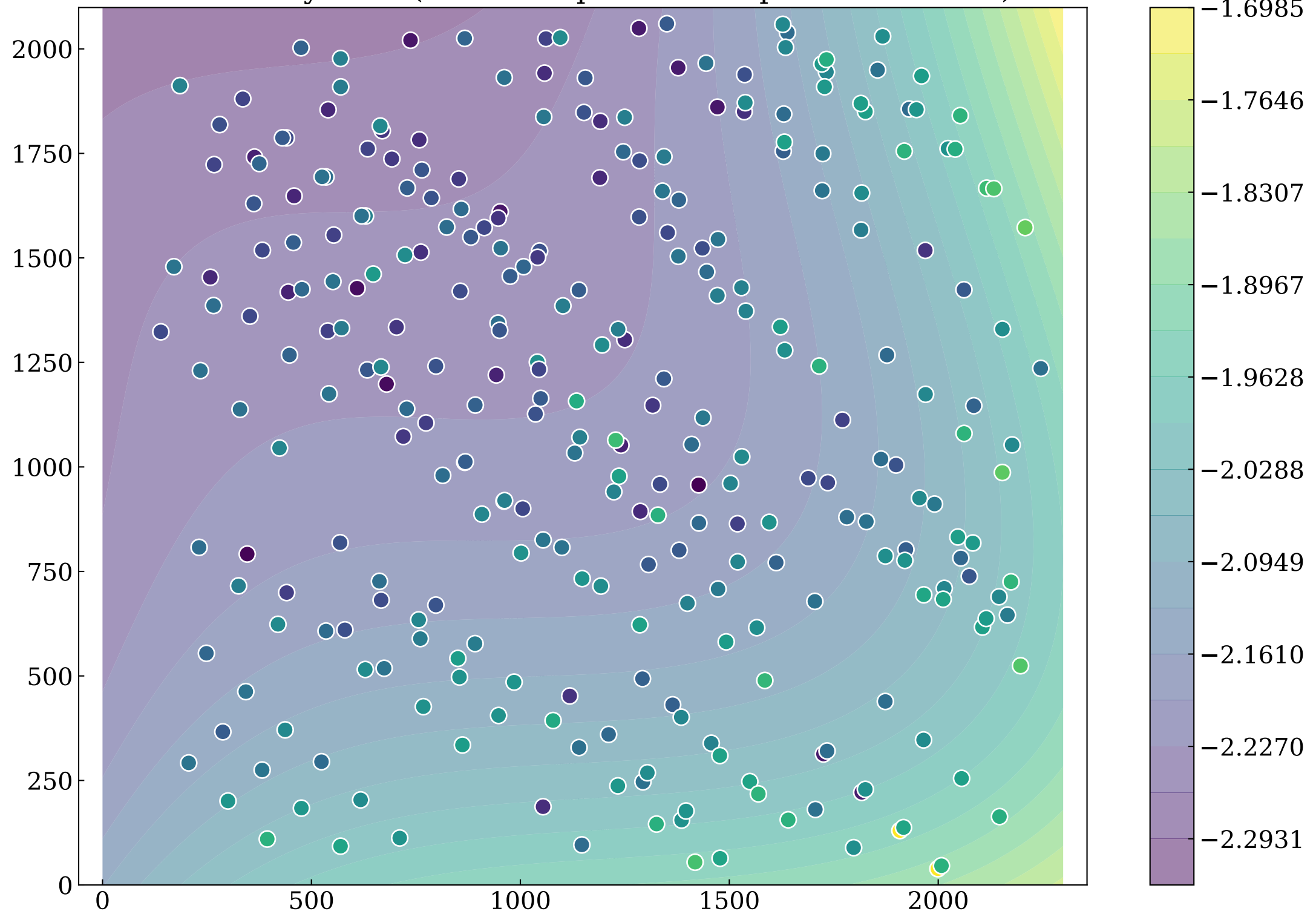
Module A yoffset (to actual spectra from predicted traces)
