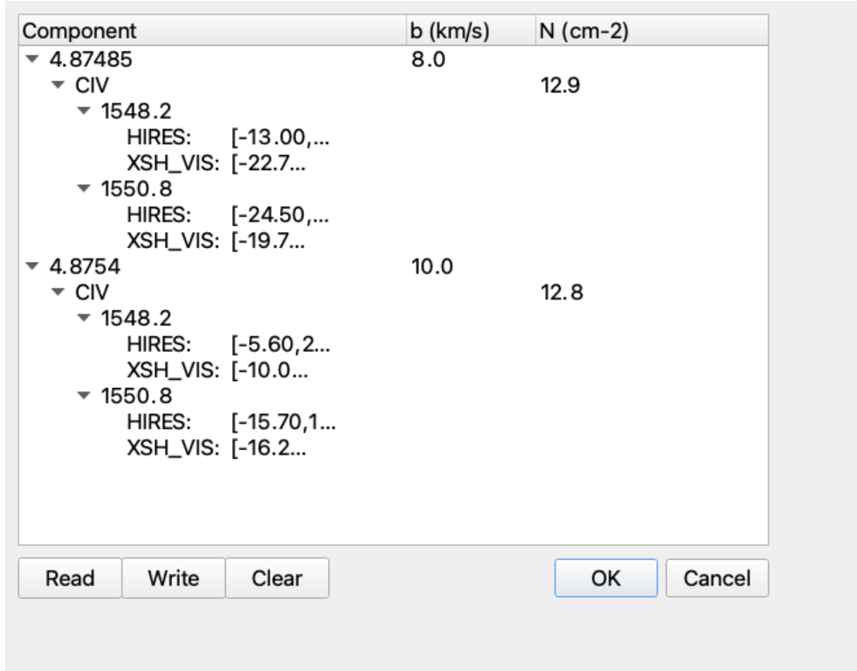
Figure 4: Figure 4: VP Model Tree window showing the four-level hierarchy (Component at level 0, Ion at level 1, Transition at level 2, Fit Region at level 3) populated from the tutorial example. Column headers “Component”, “b (km/s)”, and “N (cm-2)” are visible.
