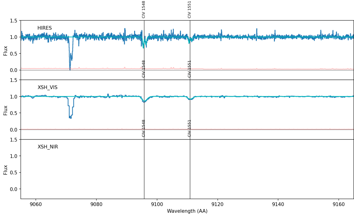
Figure 6: Figure 6: Spectrum with the cyan initial-guess Voigt profile overlaid on the C IV doublet at z = 4.875 , showing reasonable alignment with the observed absorption troughs before the MCMC fit is run.
