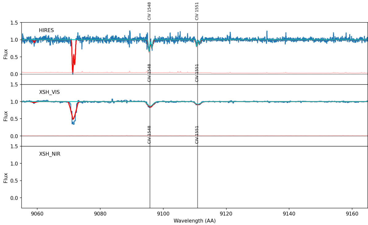
Figure 8: Figure 8: Same field as Figure 7 after additionally loading the DR1 XSH_VIS posterior profiles. The red ensemble now appears on both the HIRES and XSH_VIS panels simultaneously, providing a joint view of the constraint from two instruments.
