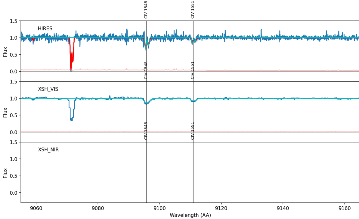
Figure 7: Figure 7: Spectrum of J0100+2802 near the C IV doublet at z = 4.875 after loading the DR1 HIRES posterior profiles. Fifty semi-transparent red draws bracket the absorption troughs, giving a direct visual impression of the posterior uncertainty.
