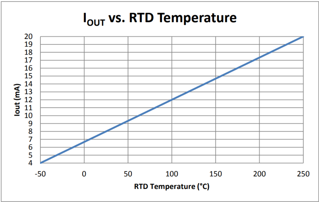
Figure 9: Output Current (I OUT ) vs. RTD Temperature
