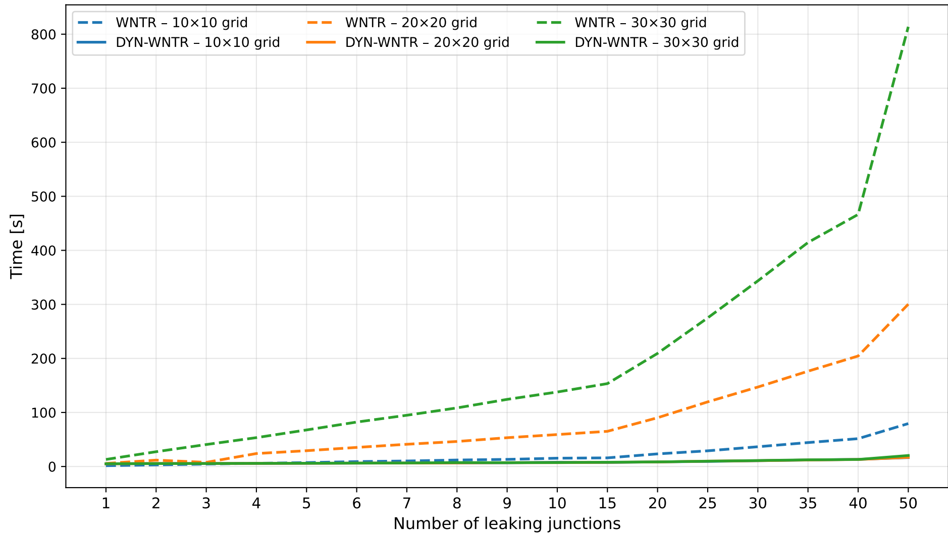
WNTR vs DYN-WNTR simulation runtime
