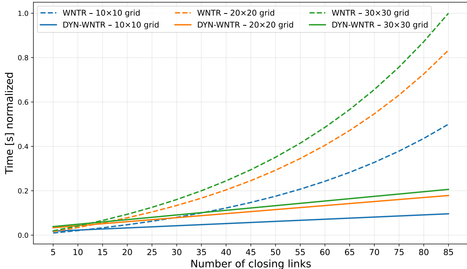
Normalized WNTR vs DYN-WNTR simulation runtime
