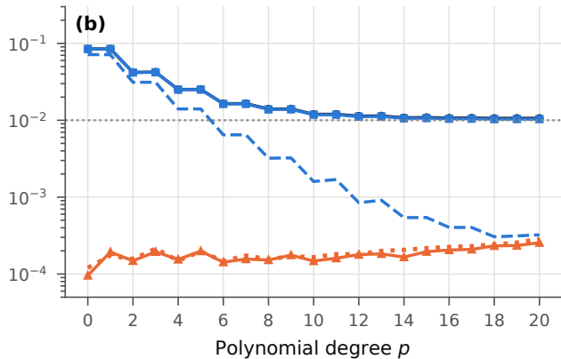
n = 1000 (800 training points)
