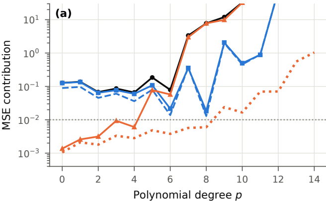
n = 100 (80 training points)
