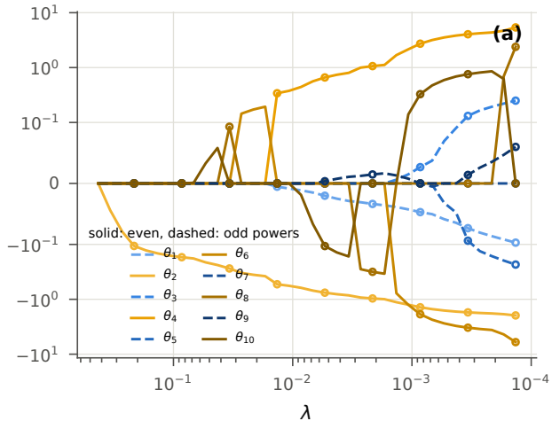
Lasso coefficient \theta_j (degree 10)
