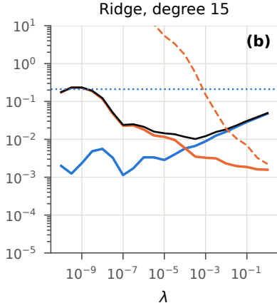
Contribution to test MSE
