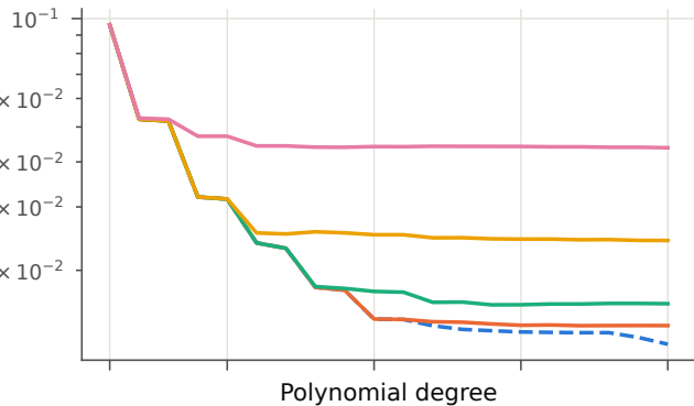
Training R^2
