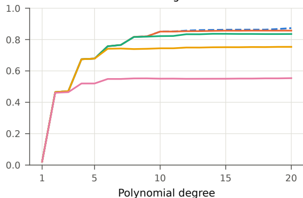
Training R^2
