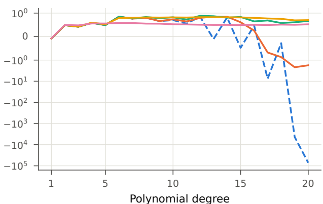
Test R^2
