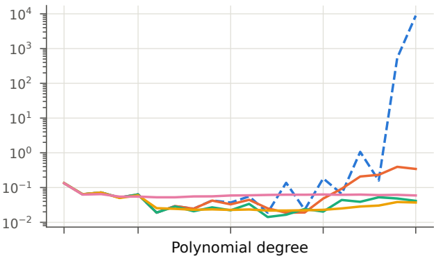
Test R^2
