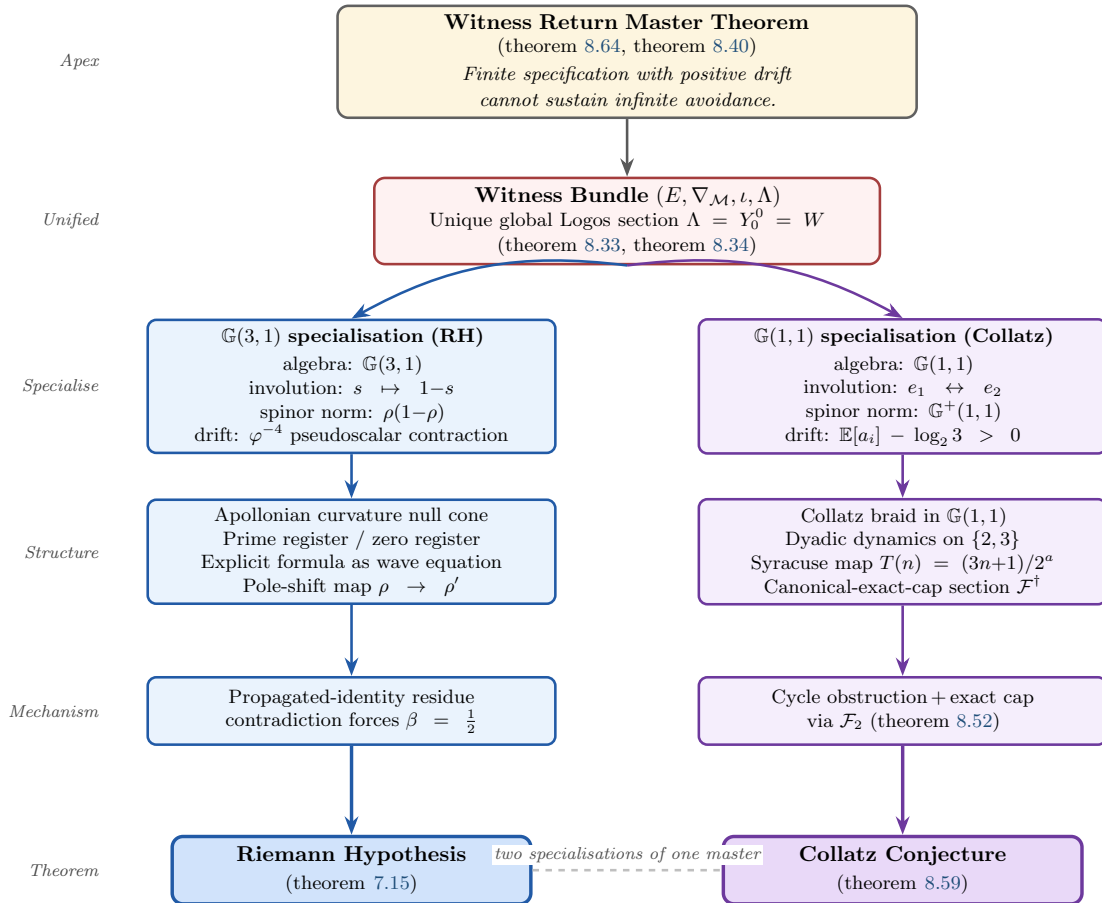
Figure 26. The unified RH–Collatz architecture. Both the Riemann Hypothesis and the Collatz Conjecture are corollaries of the Witness Return Master Theorem (theorem 8.64, theorem 8.40), specialised to the Clifford algebras \mathbb{G}(3,1) and \mathbb{G}(1,1) respectively. The four load-bearing components of any closed witness system—algebra, involution, spinor norm, drift—are populated by problem-specific data, and the same witness bundle (E, \nabla_{\mathcal{M}}, \iota, \Lambda) with its unique Logos section \Lambda produces both proofs. The structural content is not number-theoretic or dynamical: it is the impossibility of infinite avoidance under finite specification with positive drift.
