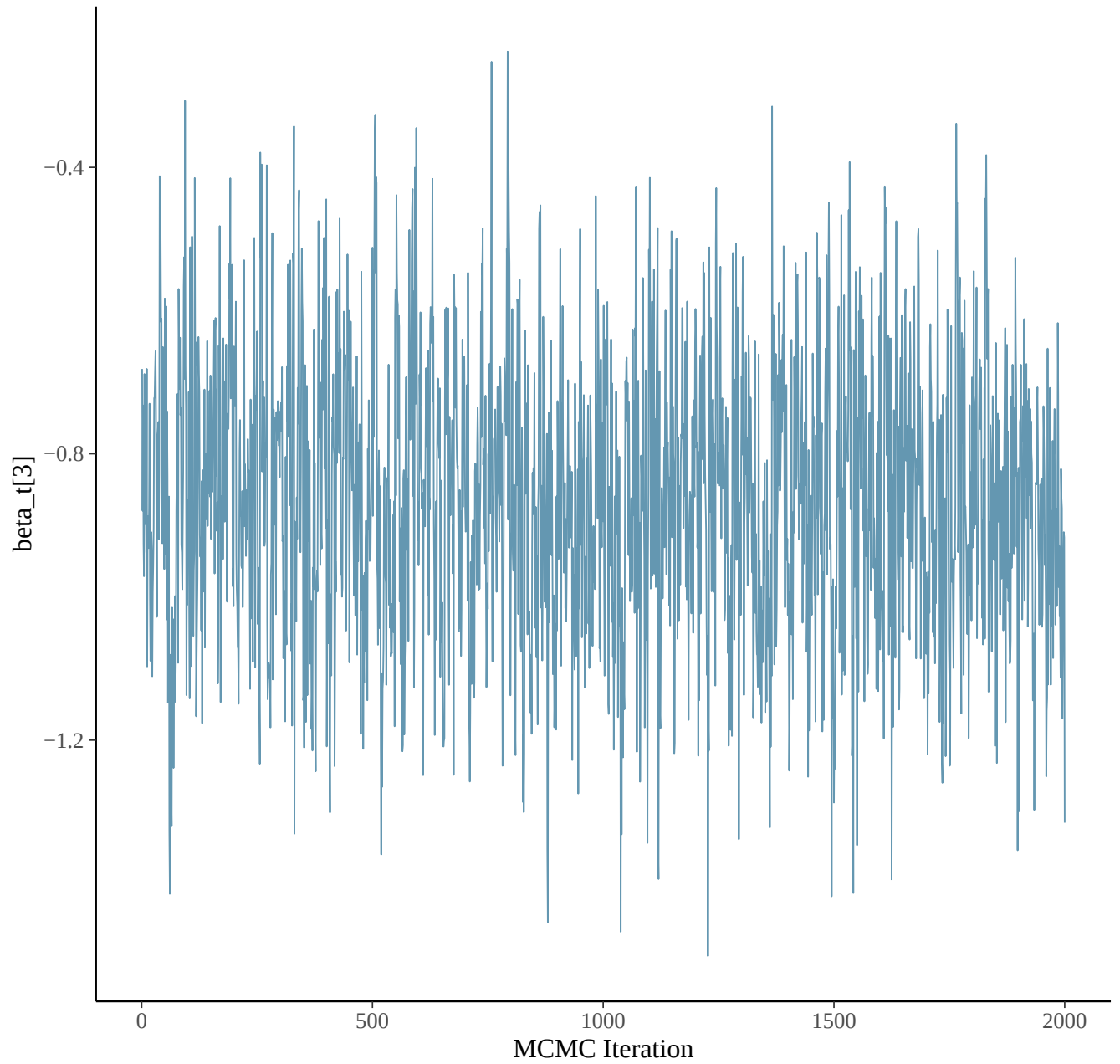
Trace Plot for \text{beta}_t[3]
