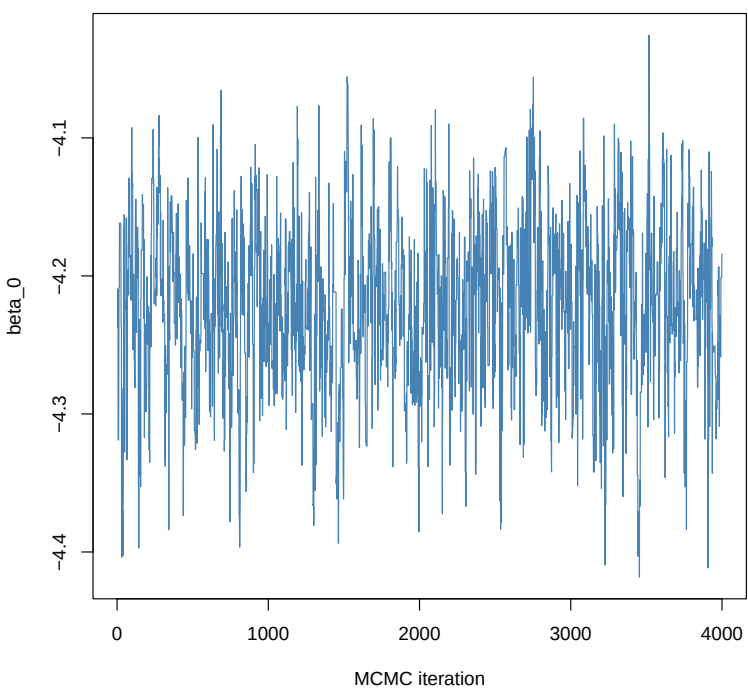
Trace Plot for beta_0
