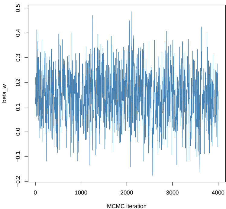
Trace Plot for beta_w
