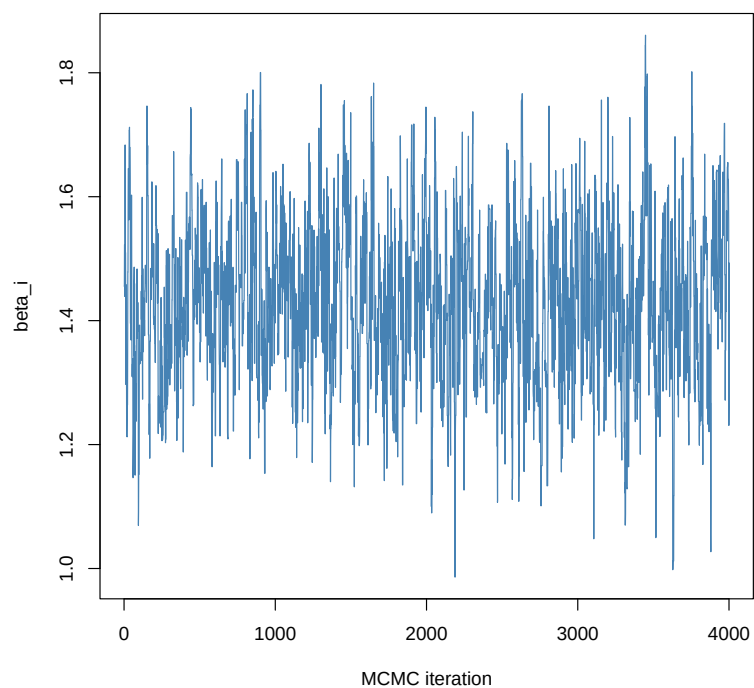
Trace Plot for beta_i
