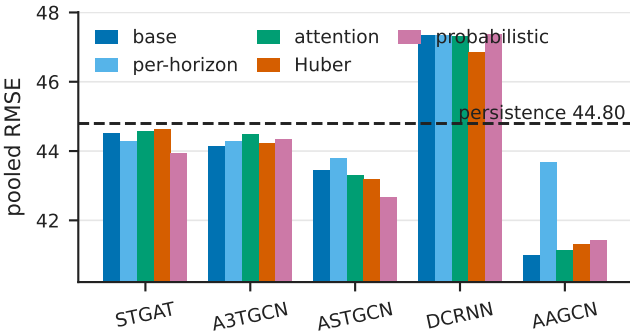
(a) all windows
