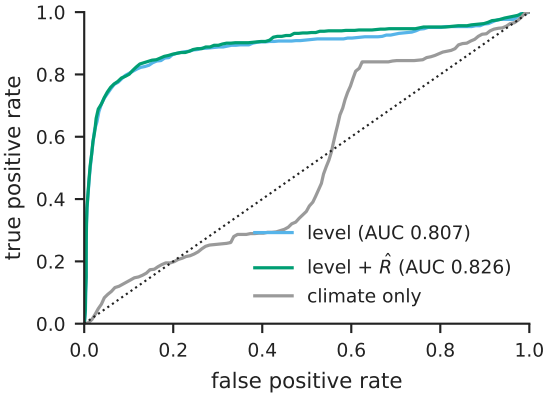
(a) ROC, 3 weeks ahead (base rate 14.4%)
