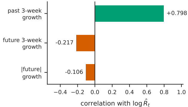
(b) \hat{R} looks backwards
