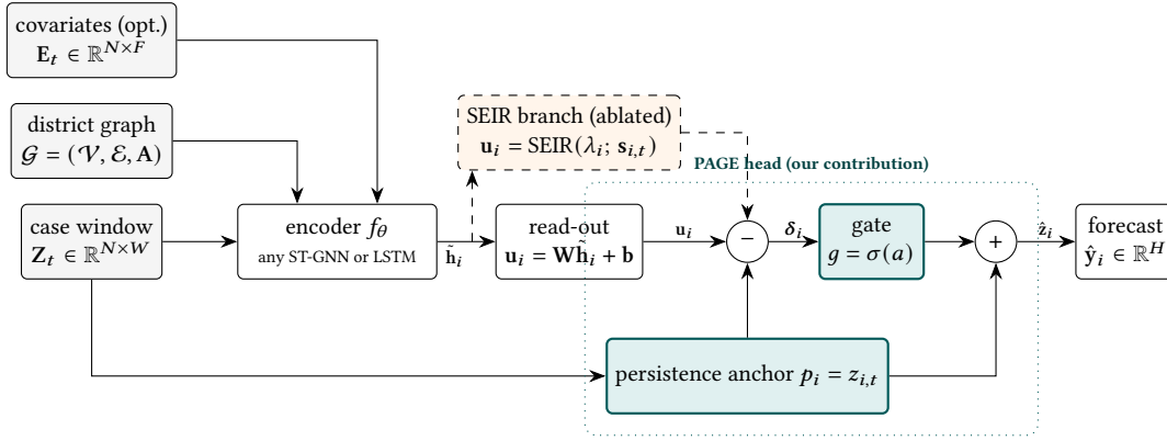
Figure 1: PAGE. An unchanged encoder reads the last W weeks of standardised log cases on the district graph. Its read-out u_i is turned into a departure \delta_i = u_i - p_i \mathbf{1} from the persistence anchor, shrunk by a learned gate, and added back to the anchor. The dashed SEIR branch replaces the read-out with a differentiable simulator; it is the component the ablation removes.
