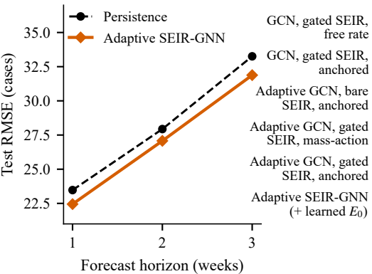
(a) Error by horizon
