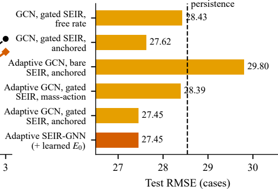
(b) SEIR-head variants
