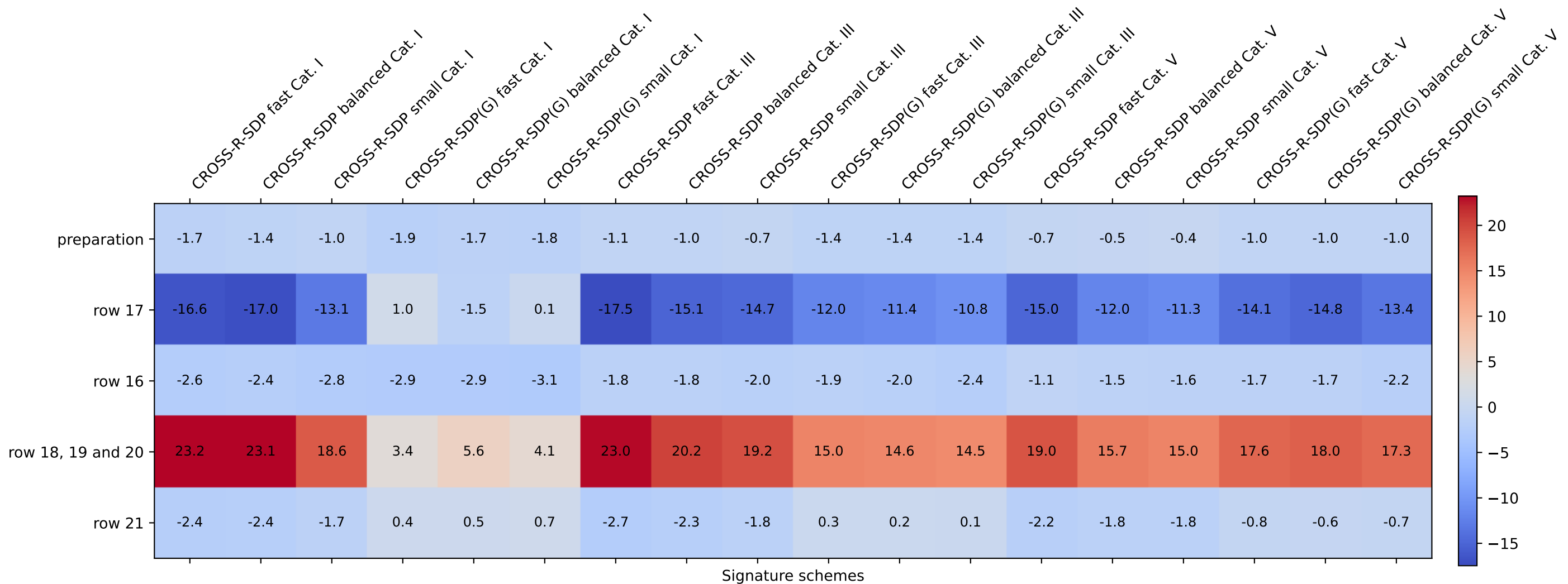
Heatmap of CROSS signature loop 1
