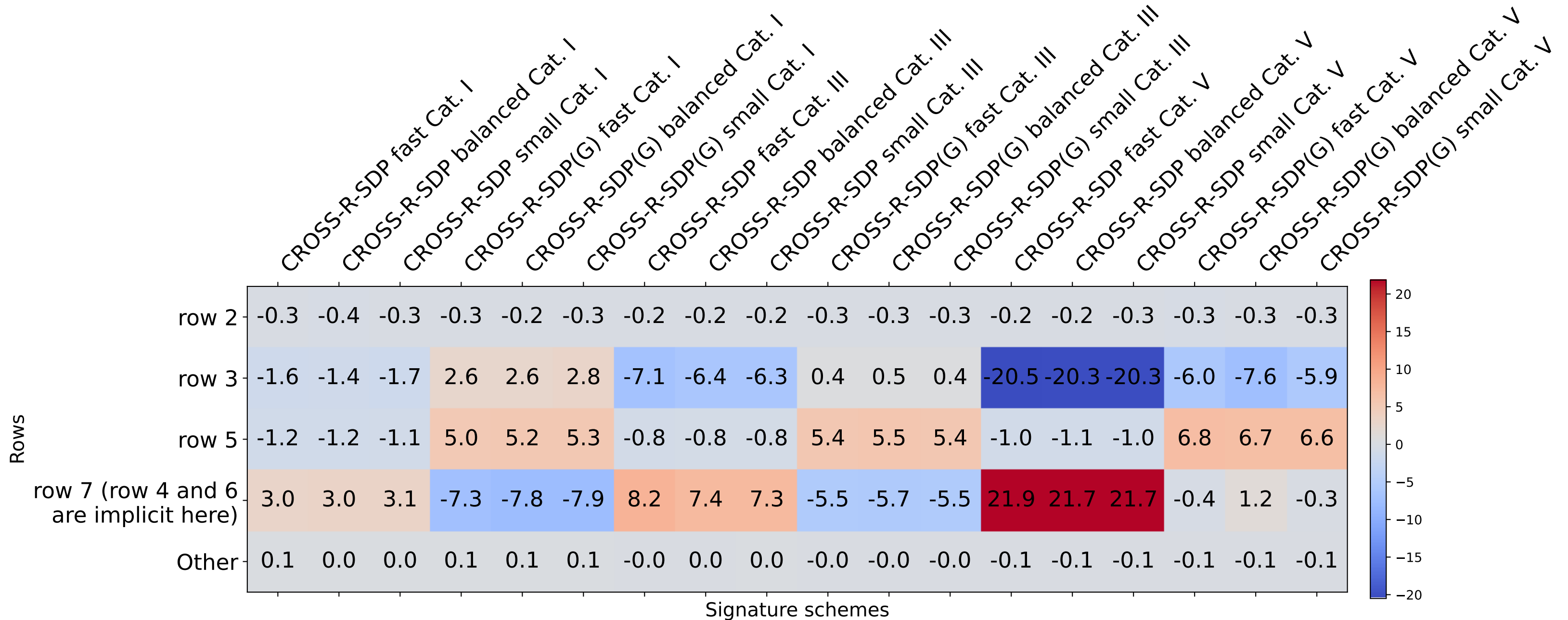
Heatmap of CROSS key generation internal analysis
