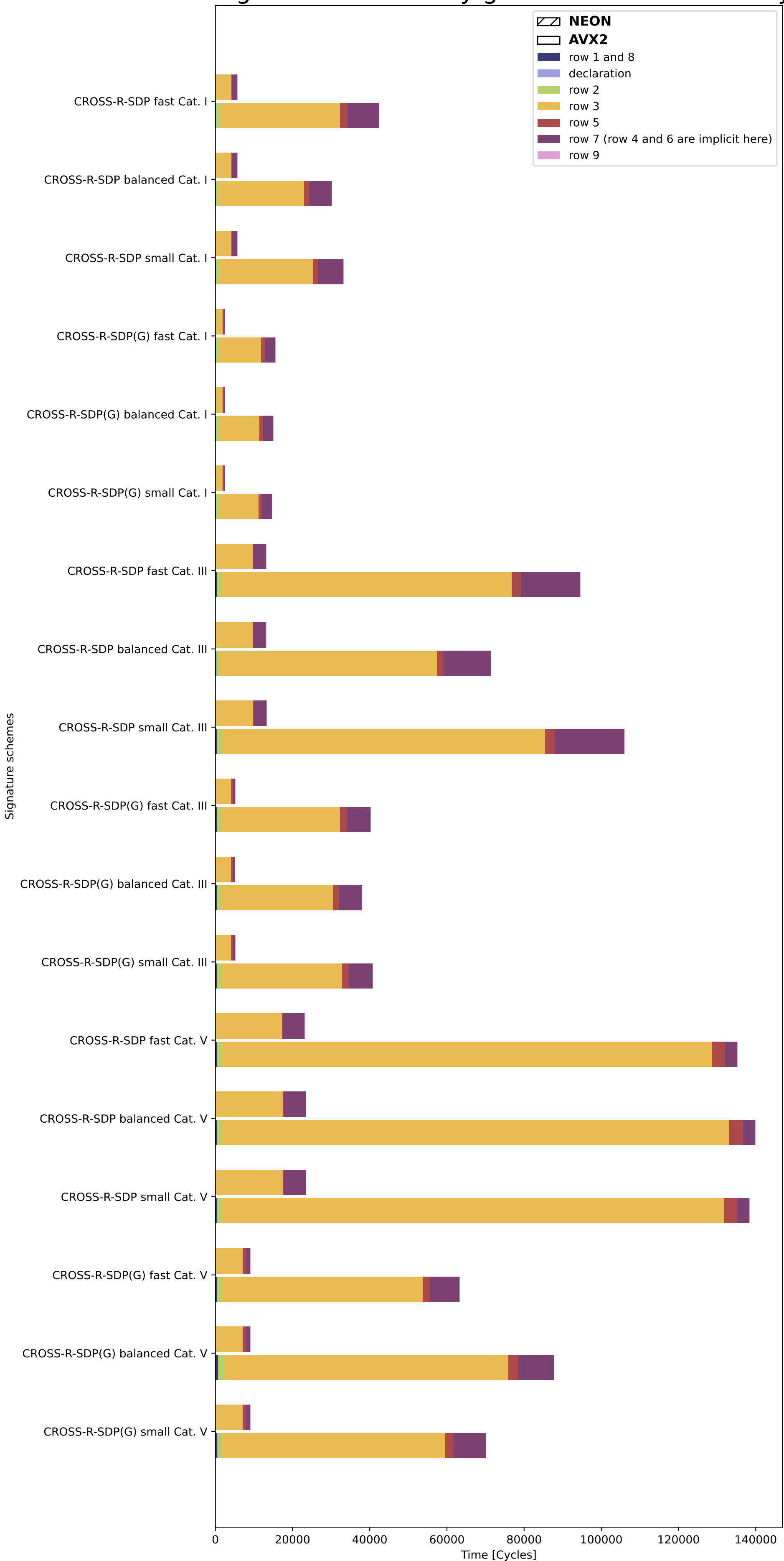
Histogram of CROSS key generation internal analysis
