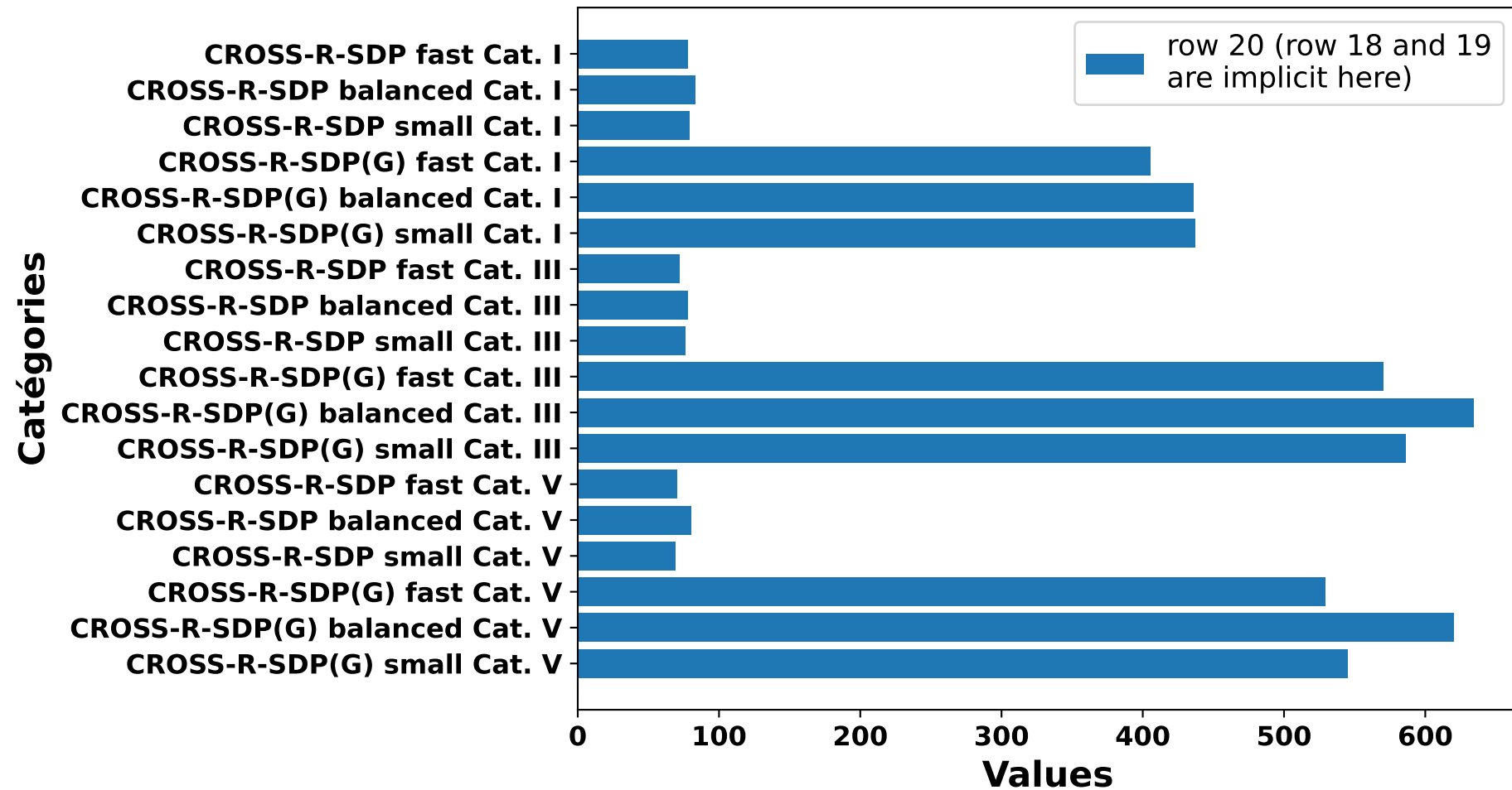
Histogram of CROSS signature loop 2 AVX2
