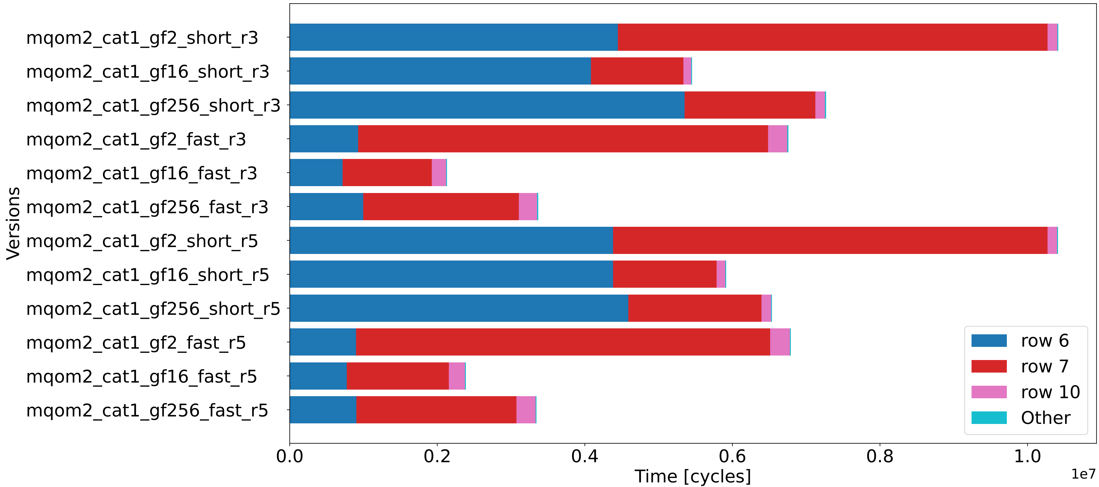
Histogram of MQOMV2.1 signature internal analysis AVX2 CAT. I
