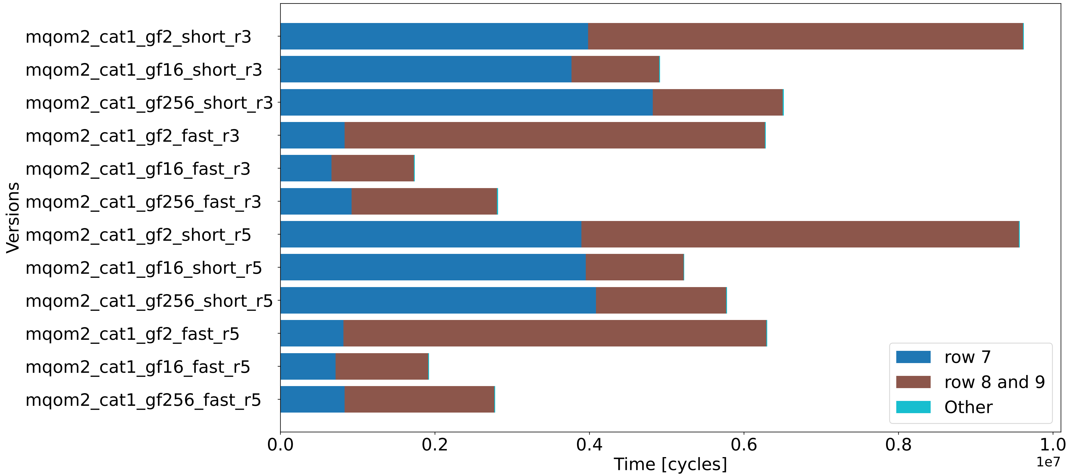
Histogram of MQOMV2.1 verification internal analysis AVX2 CAT. I
