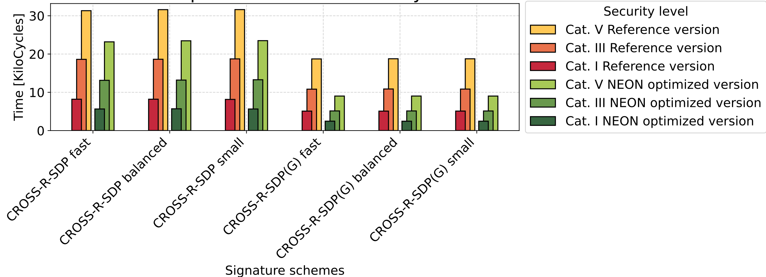
Histogram of CROSS key generation Reference version and NEON optimized version in kilocycle
