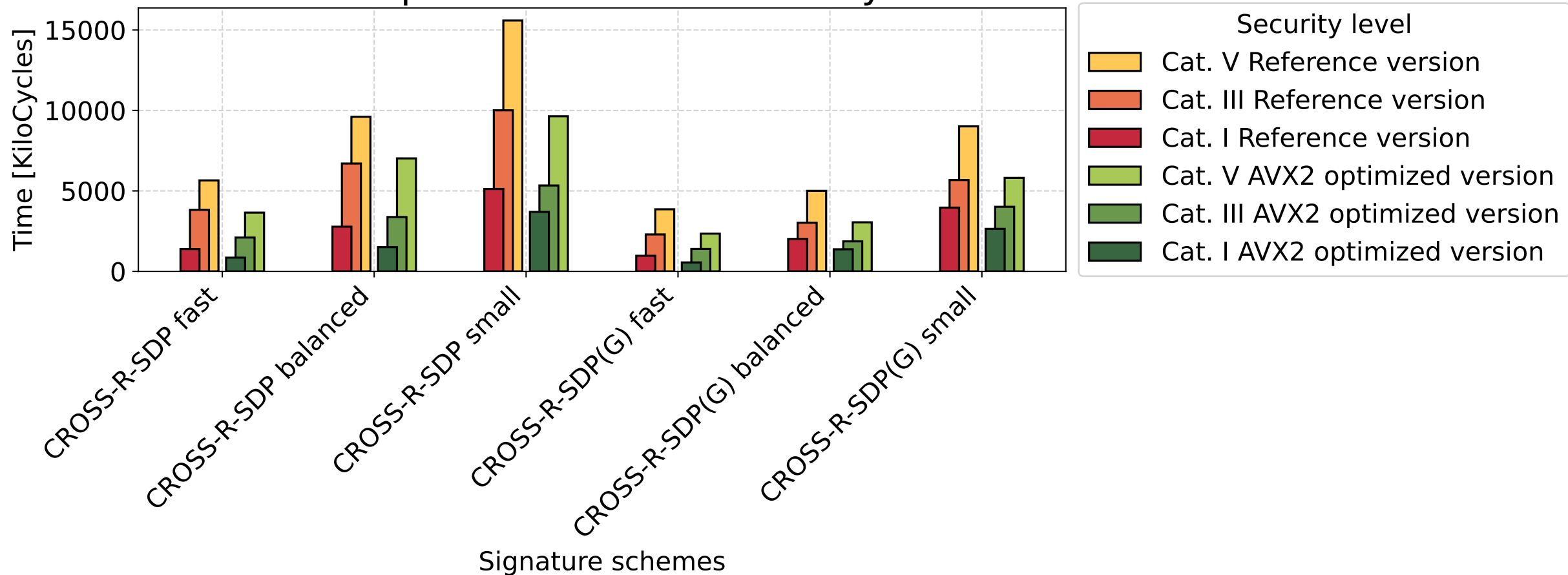
Histogram of CROSS signature Reference version and AVX2 optimized version in kilocycle
