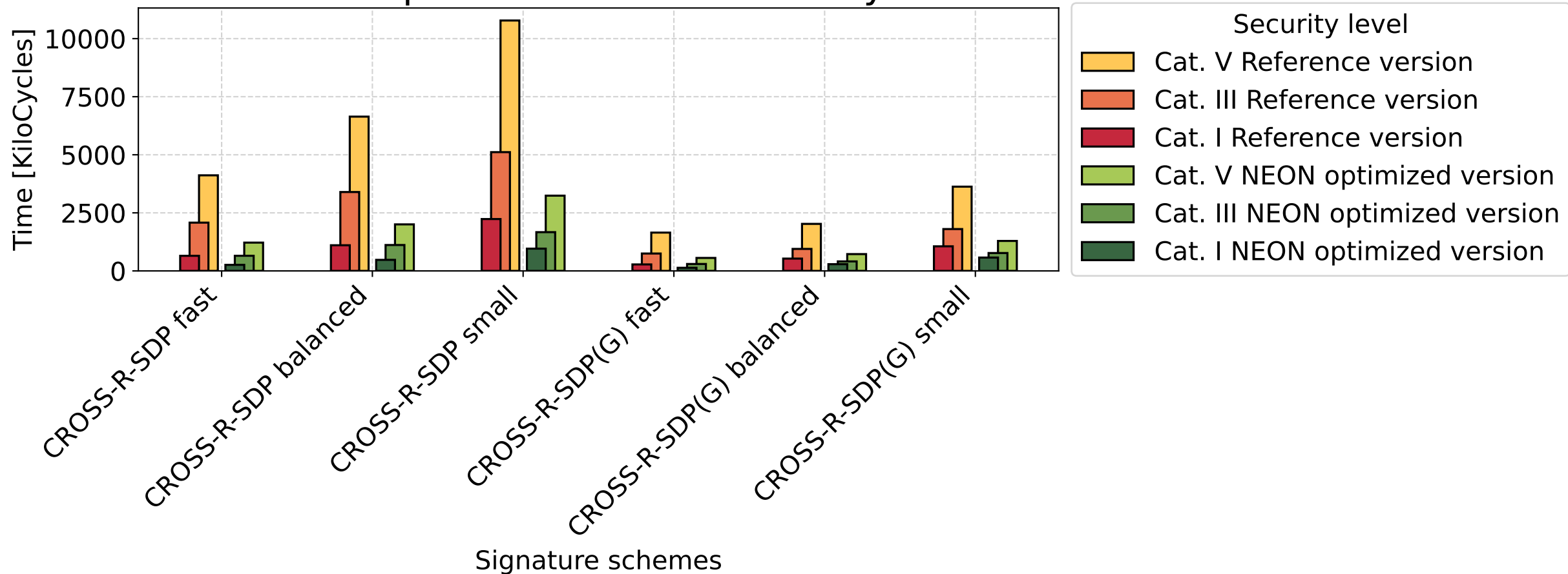
Histogram of CROSS signature Reference version and NEON optimized version in kilocycle
