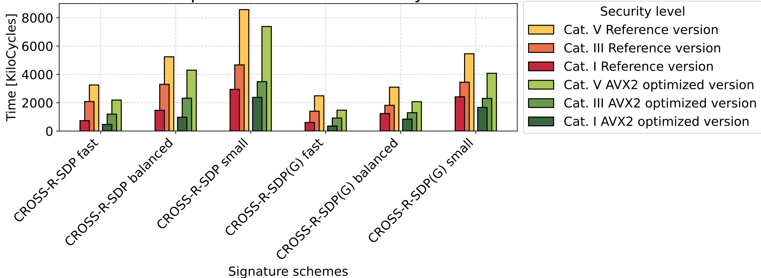
Histogram of CROSS verification Reference version and AVX2 optimized version in kilocycle
