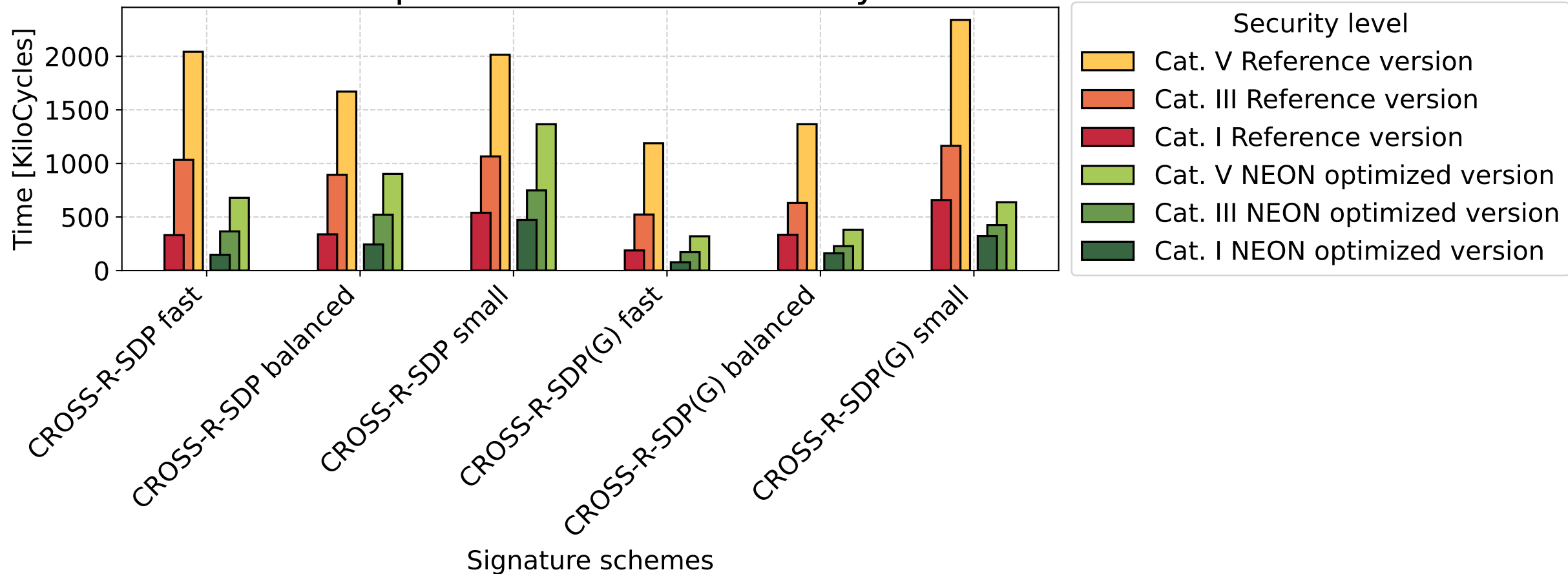
Histogram of CROSS verification Reference version and NEON optimized version in kilocycle
