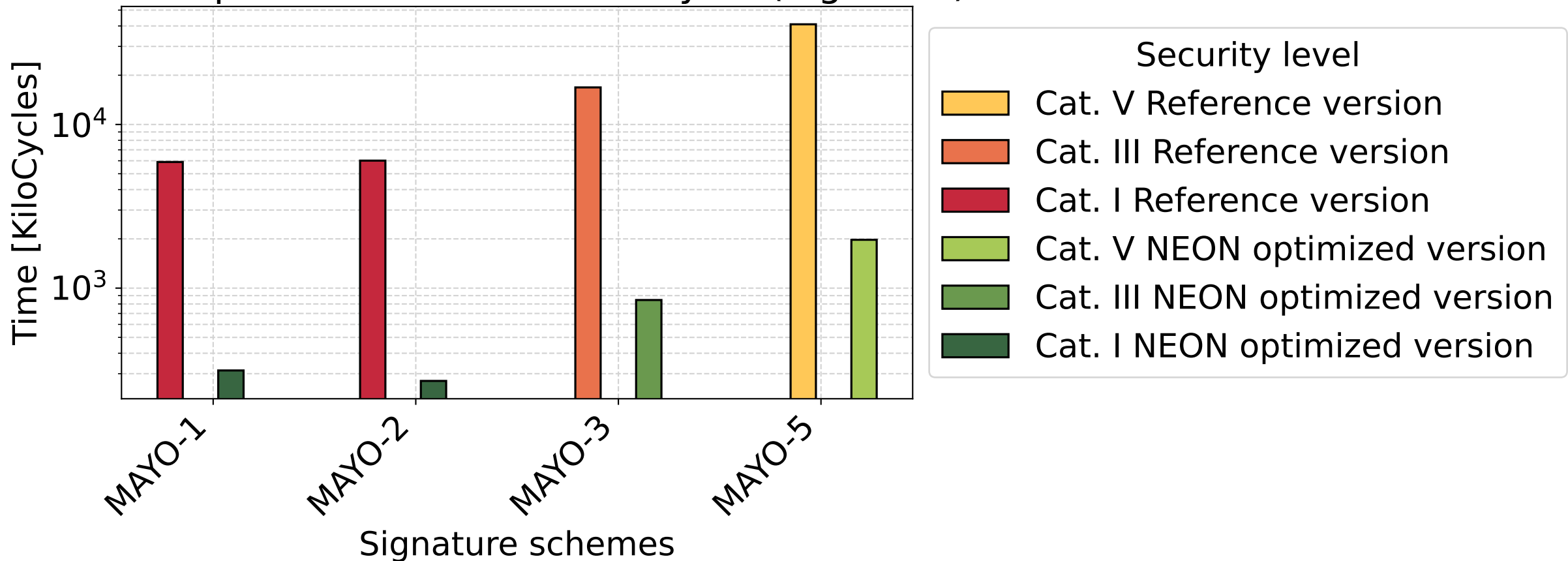
Histogram of MAYO key generation Reference version and NEON optimized version in kilocycle (log scale)
