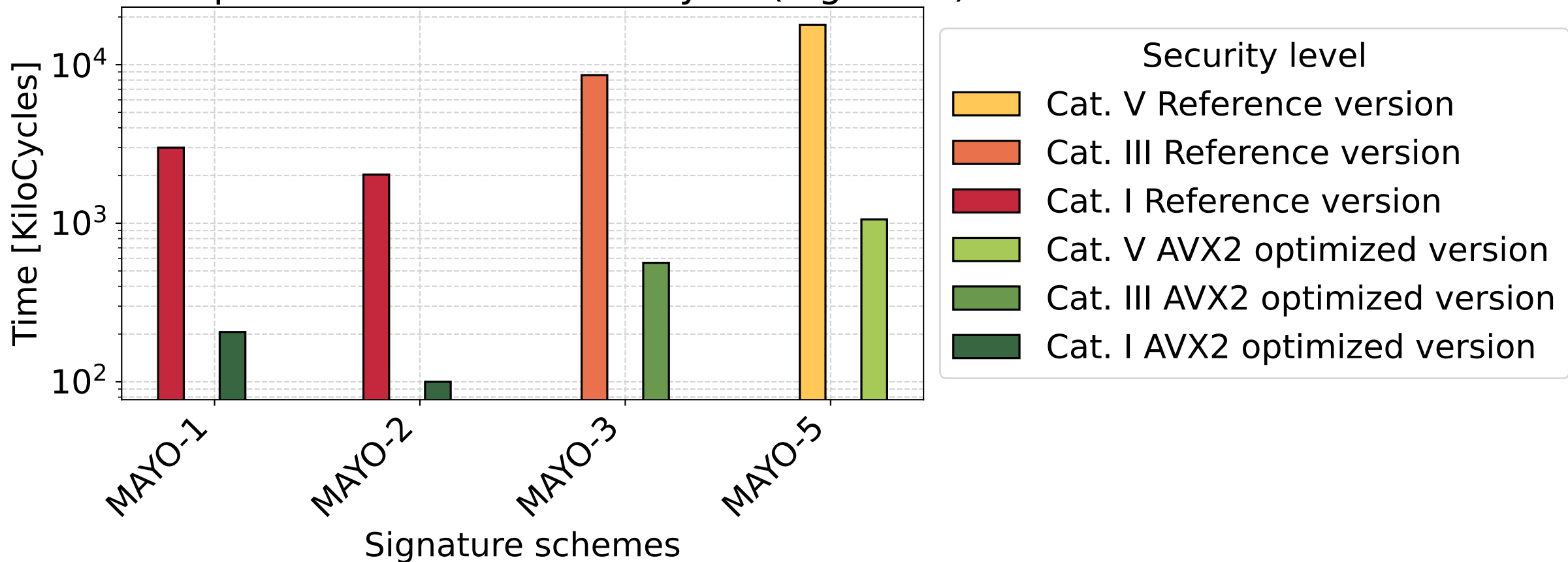
Histogram of MAYO signature Reference version and AVX2 optimized version in kilocycle (log scale)
