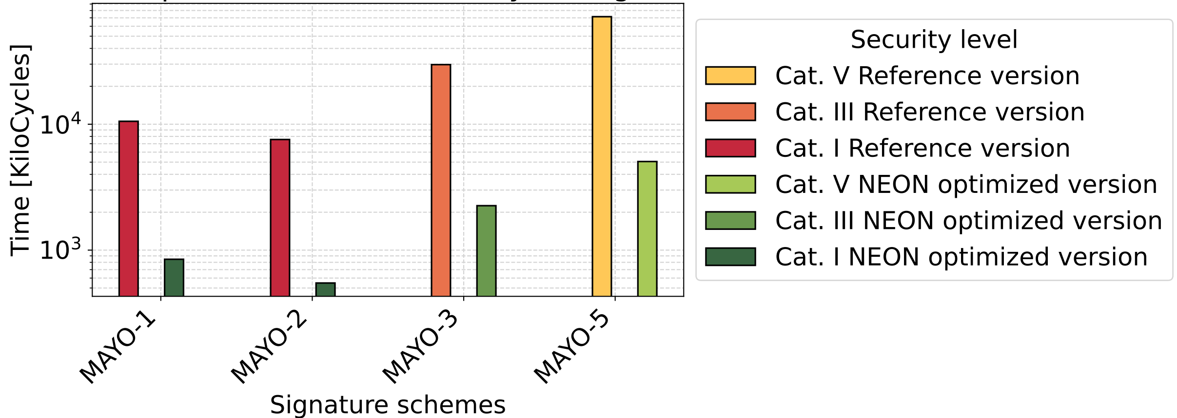
Histogram of MAYO signature Reference version and NEON optimized version in kilocycle (log scale)
