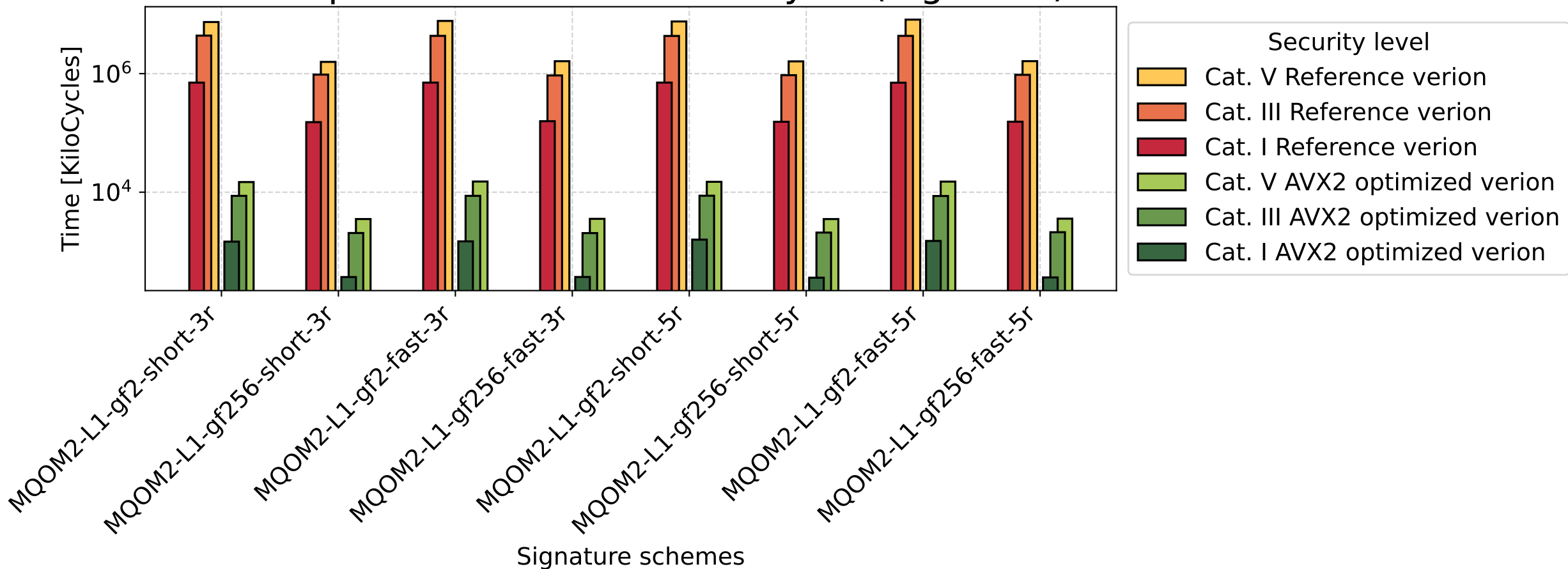
Histogram of MQOM key generation Reference version and AVX2 optimized version in kilocycle (log scale)
