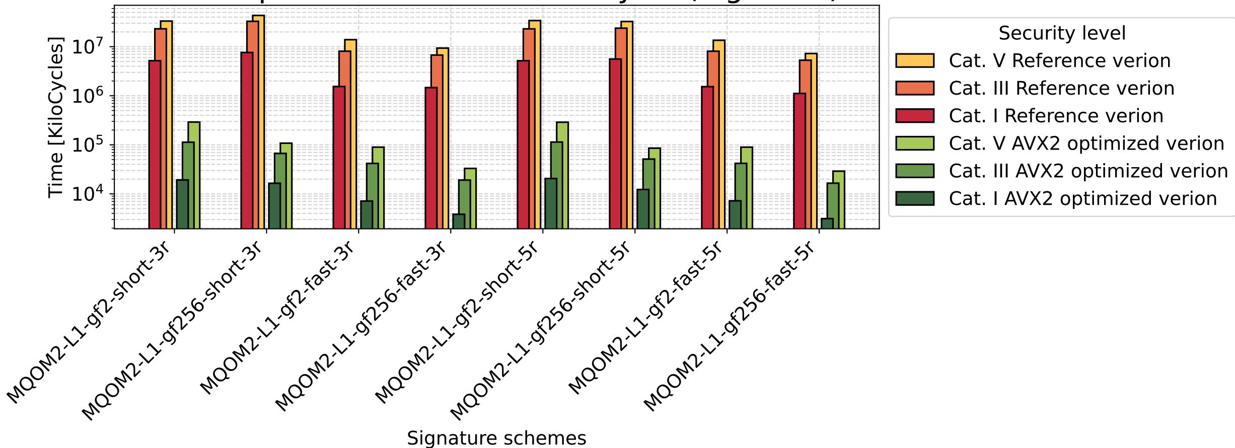
Histogram of MQOM verification Reference version and AVX2 optimized version in kilocycle (log scale)
