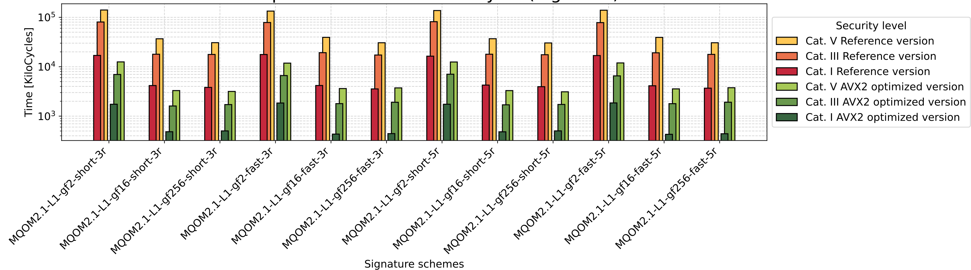
Histogram of MQOMv2.1 key generation Reference version and AVX2 optimized version in kilocycle (log scale)
