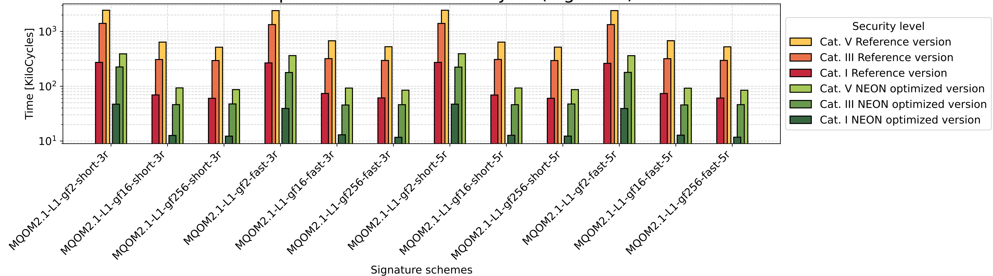
Histogram of MQOMv2.1 key generation Reference version and NEON optimized version in kilocycle (log scale)
