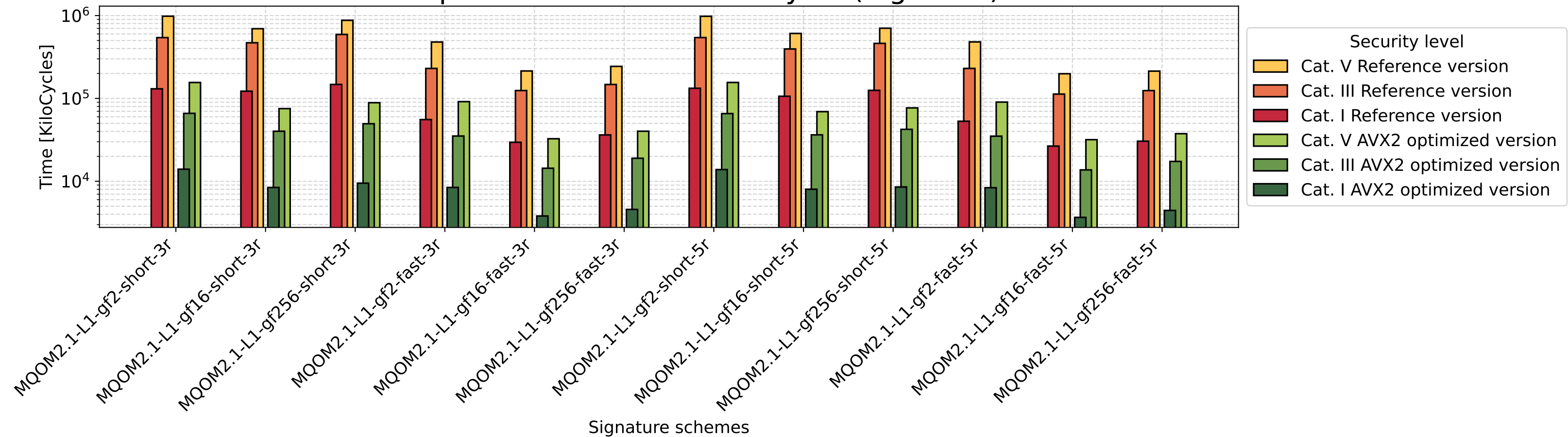
Histogram of MQOMv2.1 signature Reference version and AVX2 optimized version in kilocycle (log scale)
