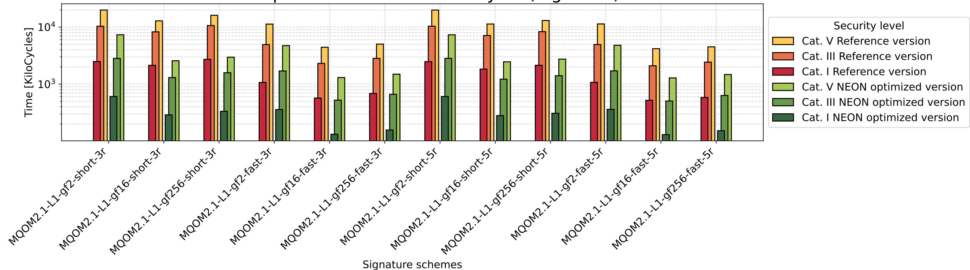
Histogram of MQOMv2.1 signature Reference version and NEON optimized version in kilocycle (log scale)
