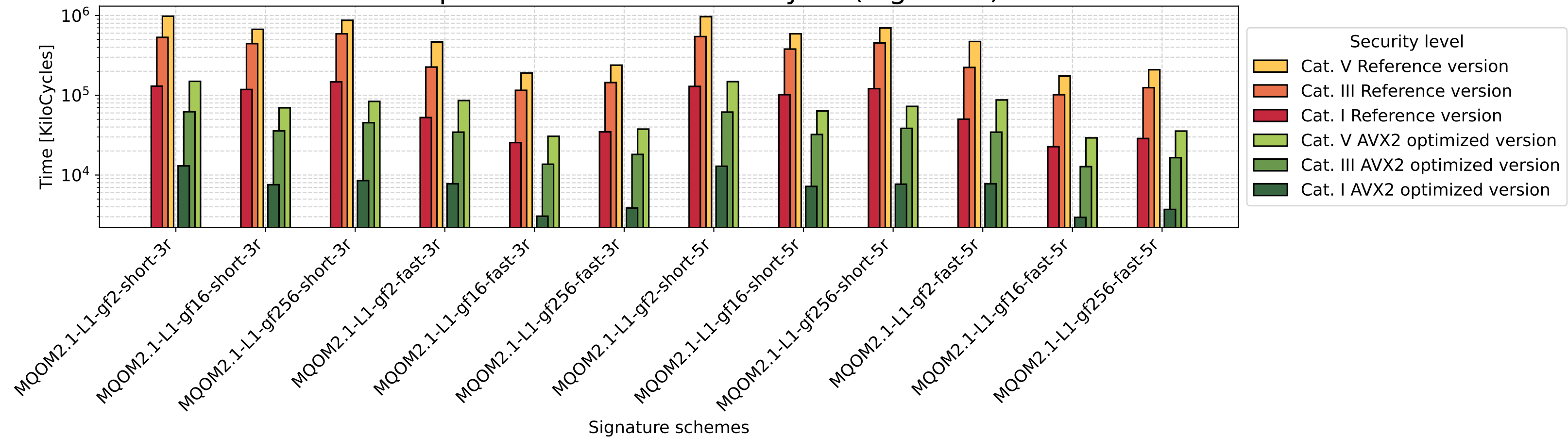
Histogram of MQOMv2.1 verification Reference version and AVX2 optimized version in kilocycle (log scale)
