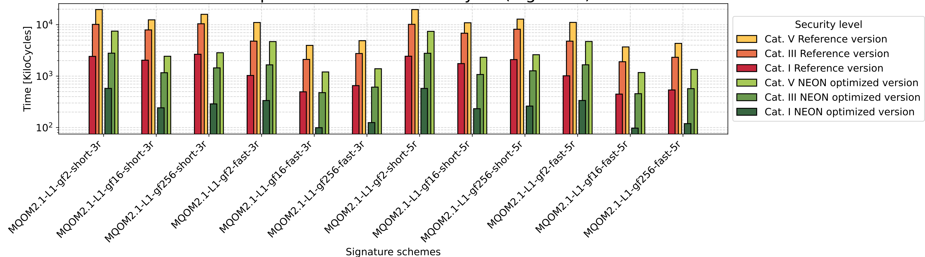
Histogram of MQOMv2.1 verification Reference version and NEON optimized version in kilocycle (log scale)
