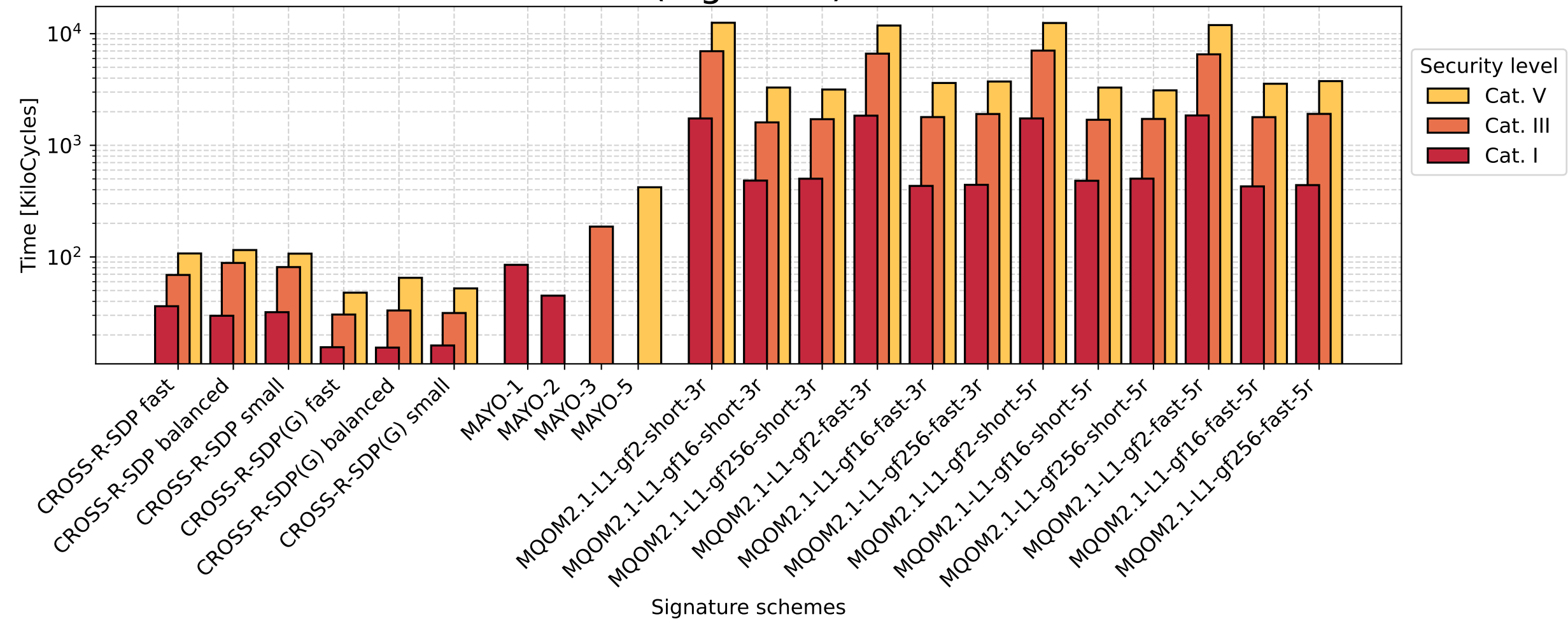
Histogram of AVX2 optimized key generation in kilocycle (log scale)
