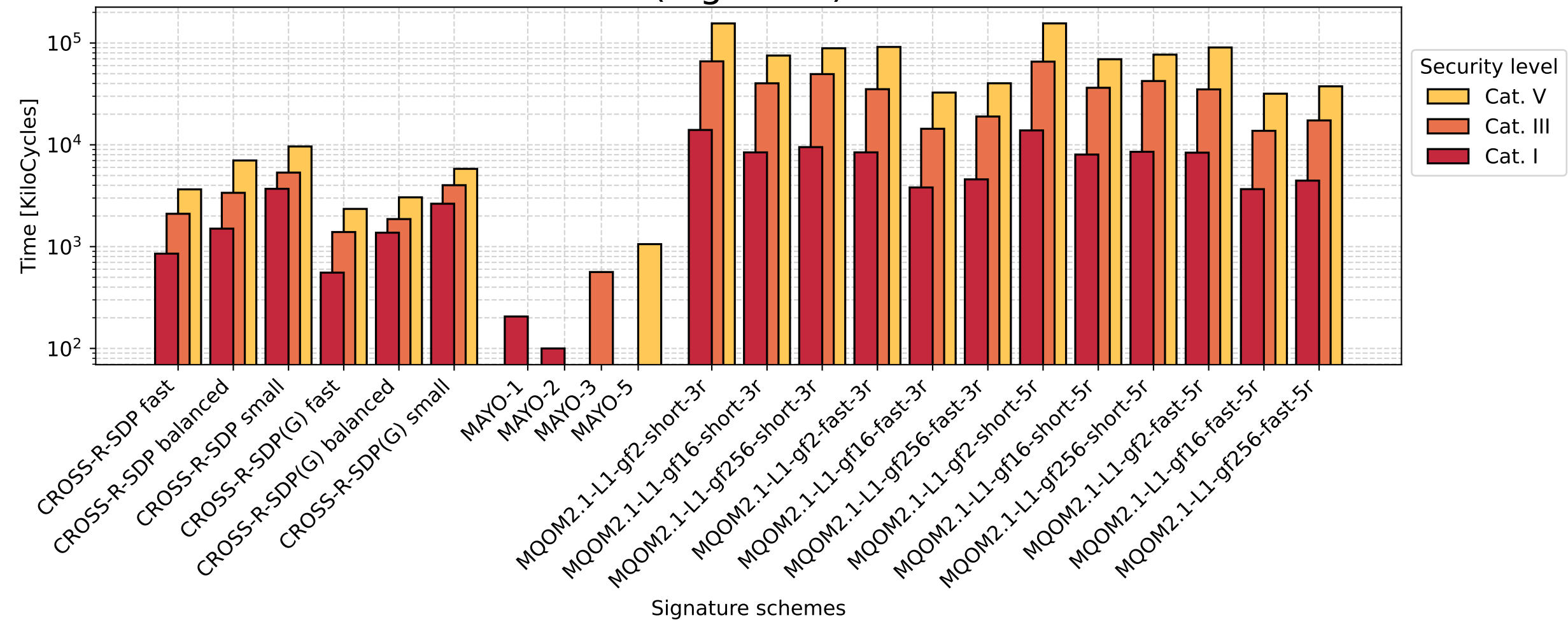
Histogram of AVX2 optimized signature in kilocycle (log scale)
