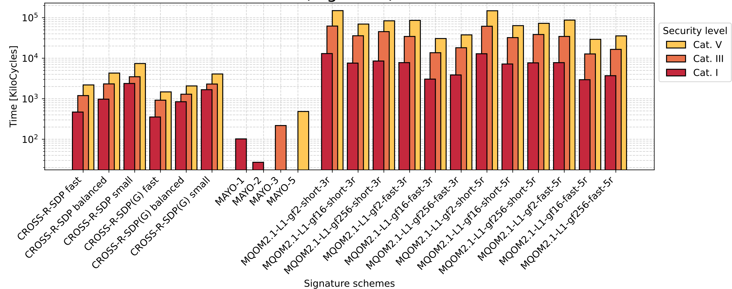
Histogram of AVX2 optimized verification in kilocycle (log scale)
