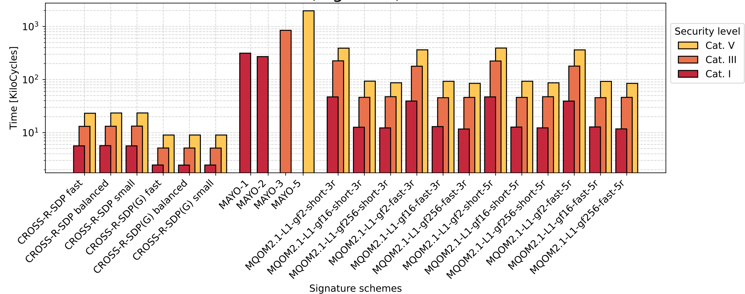
Histogram of NEON optimized key generation in kilocycle (log scale)
