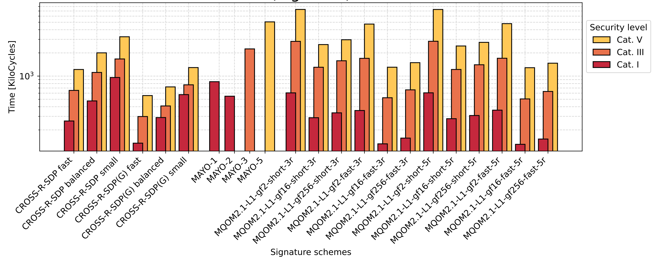
Histogram of NEON optimized signature in kilocycle (log scale)
