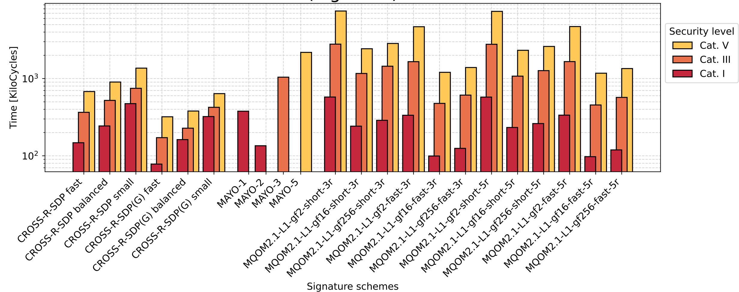
Histogram of NEON optimized verification in kilocycle (log scale)
