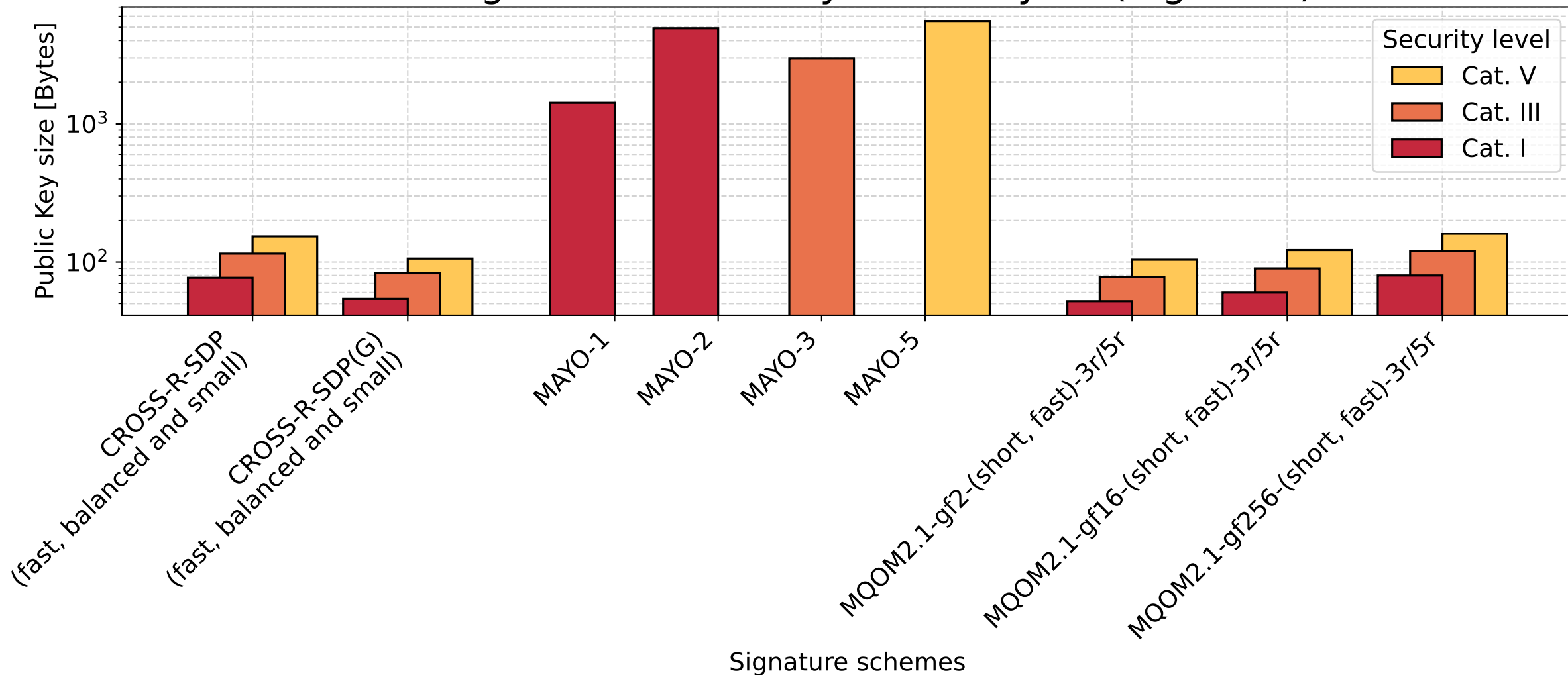
Histogram of Public Key size in Bytes (log scale)
