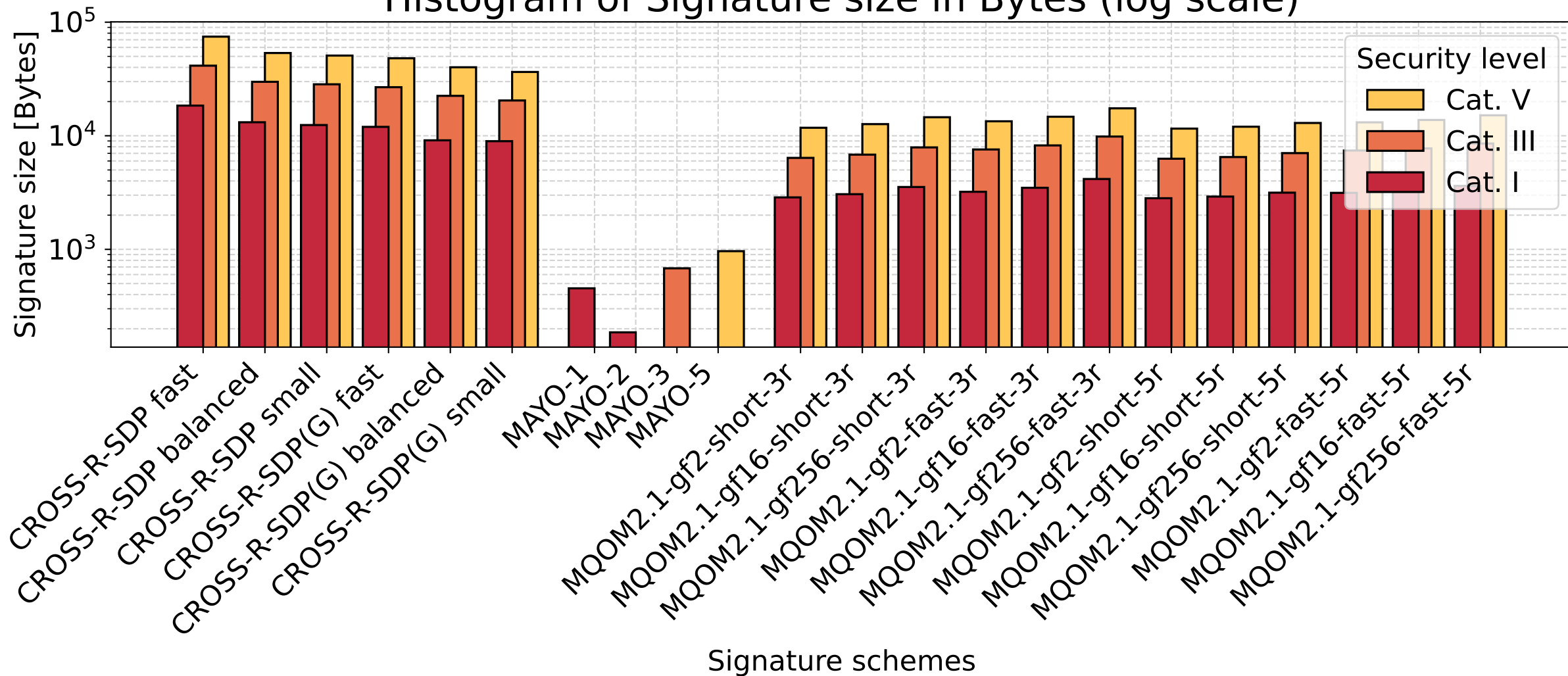
Histogram of Signature size in Bytes (log scale)
