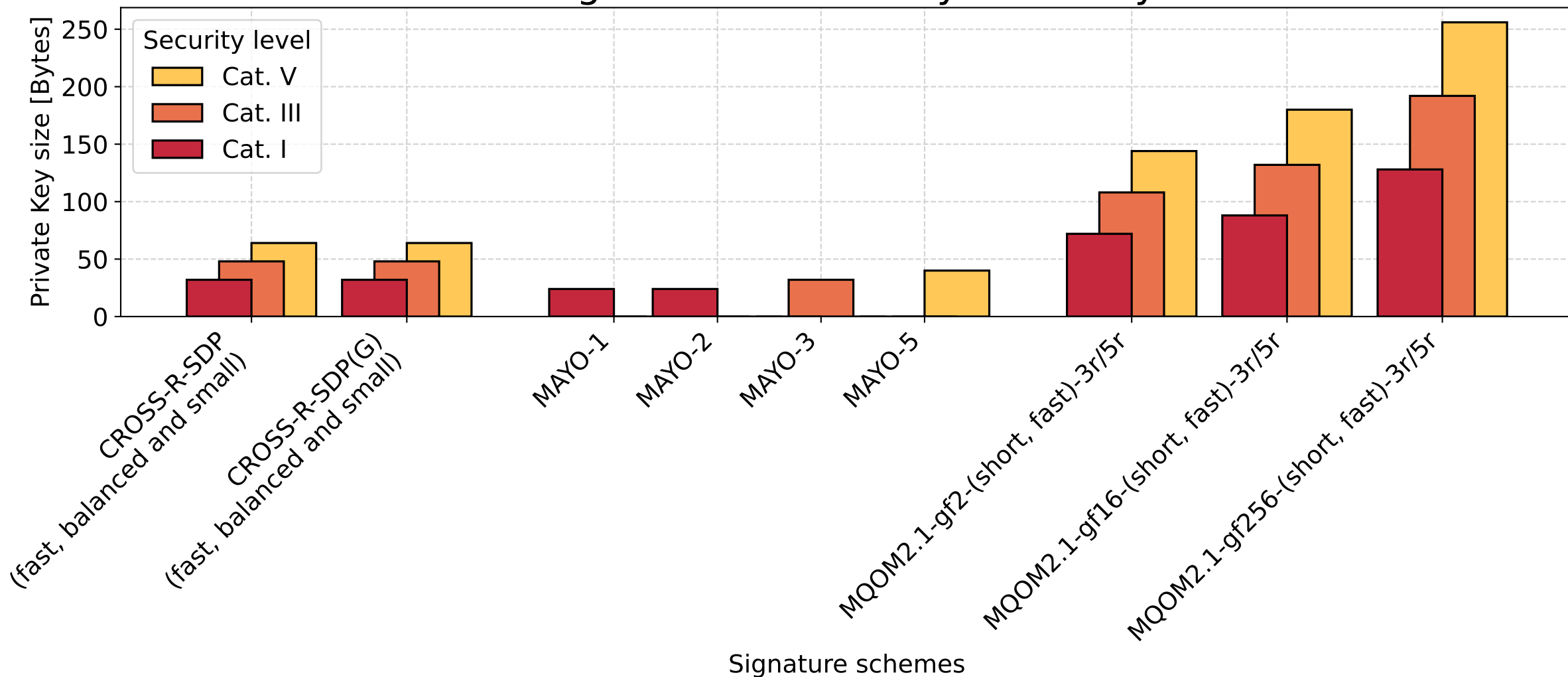
Histogram of Private Key size in Bytes
